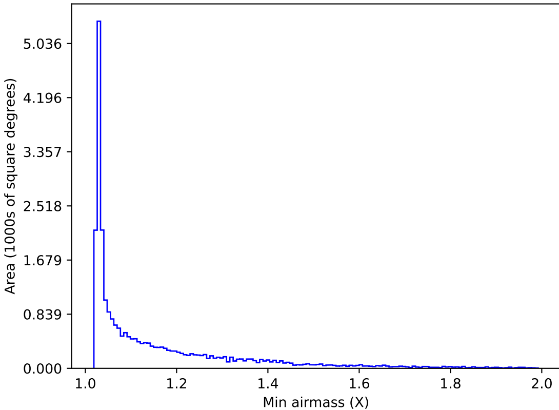
weather_cloudso35v3.4_10yrs All sky z band: Min airmass
