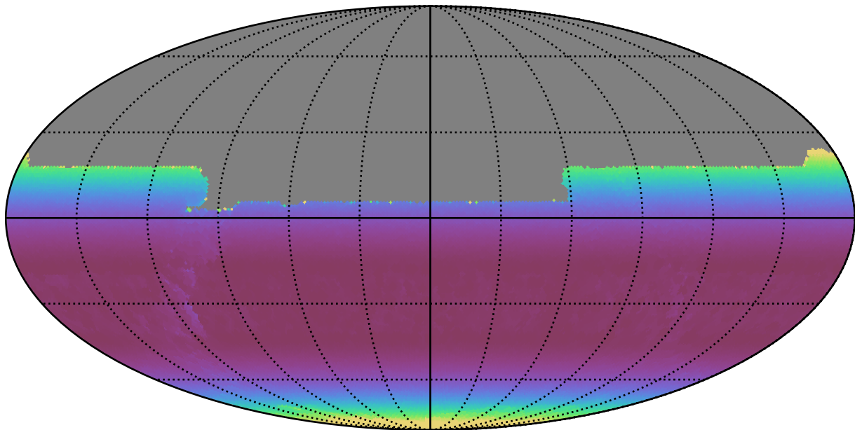
weather_cloudso35v3.4_10yrs All sky y band: Min airmass
