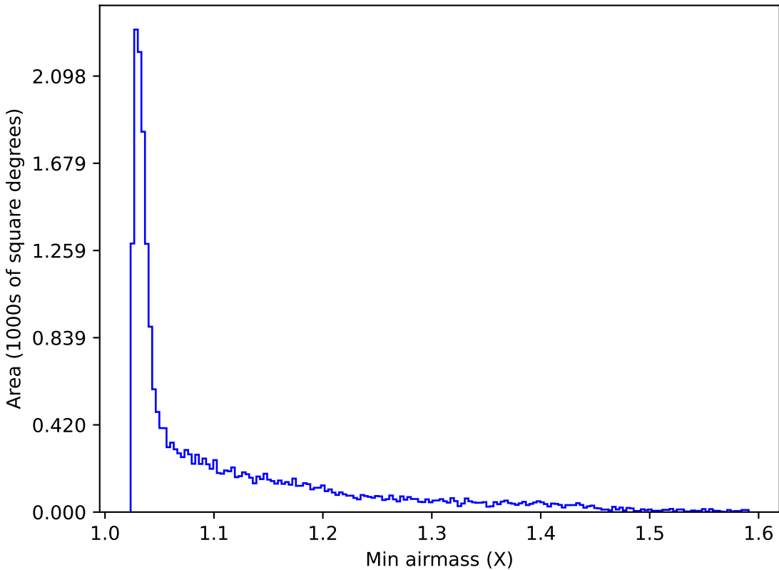
weather_cloudso35v3.4_10yrs All sky y band: Min airmass
