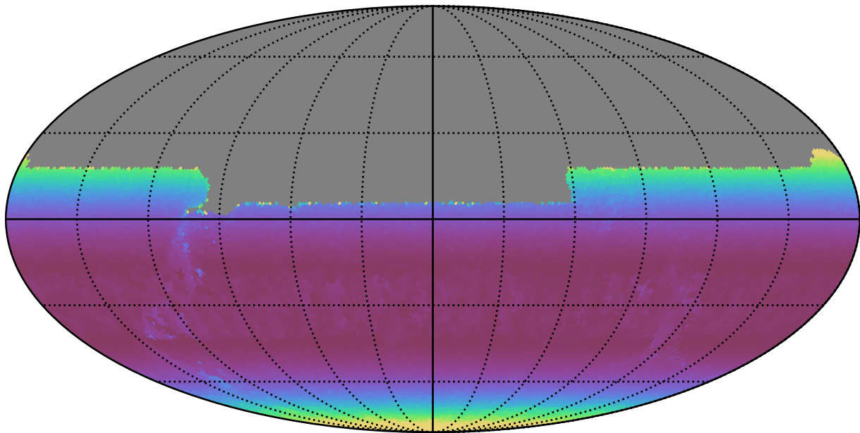
weather_cloudso35v3.4_10yrs All sky u band: Min airmass
