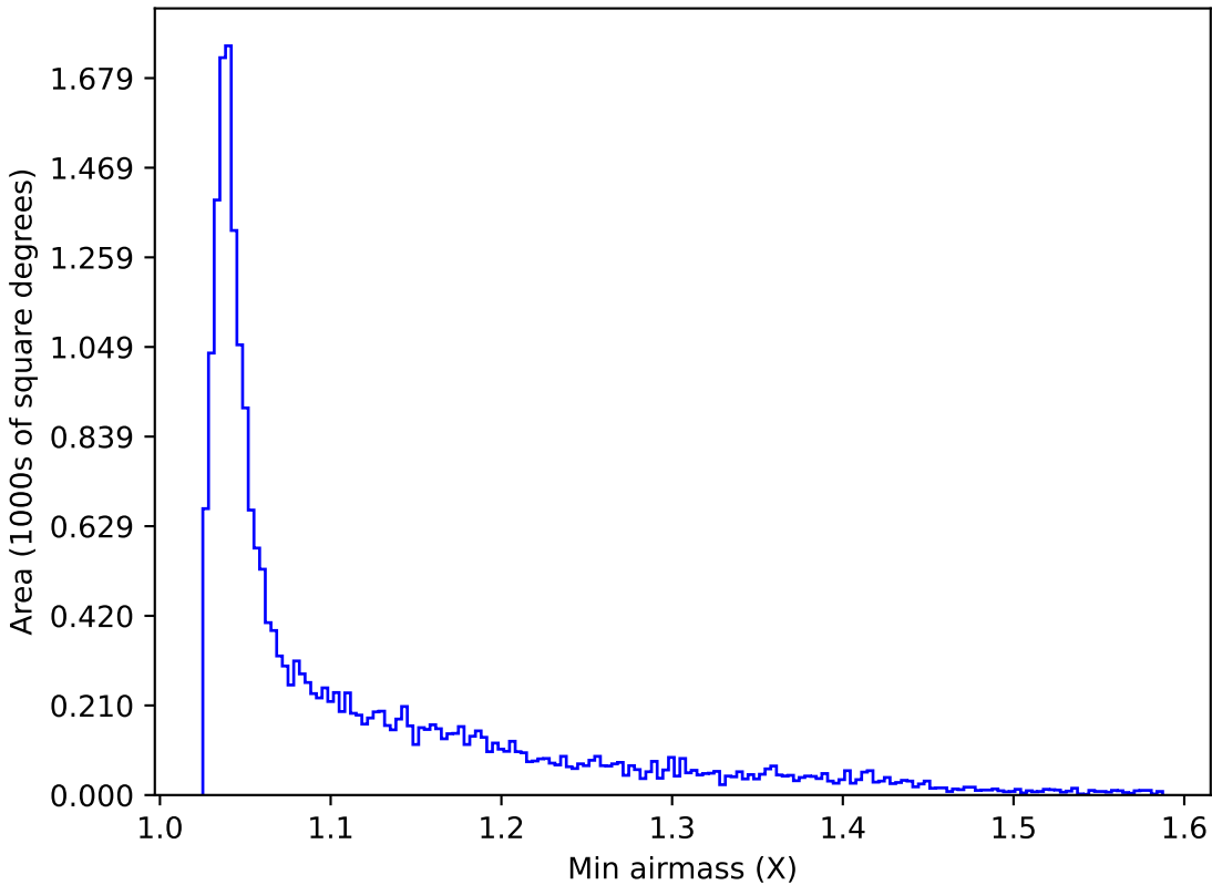
weather_cloudso35v3.4_10yrs All sky u band: Min airmass
