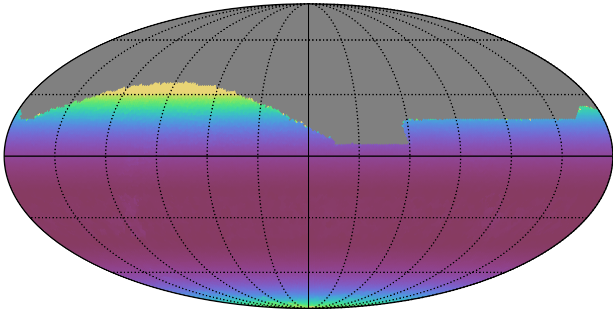
weather_cloudso35v3.4_10yrs All sky r band: Min airmass
