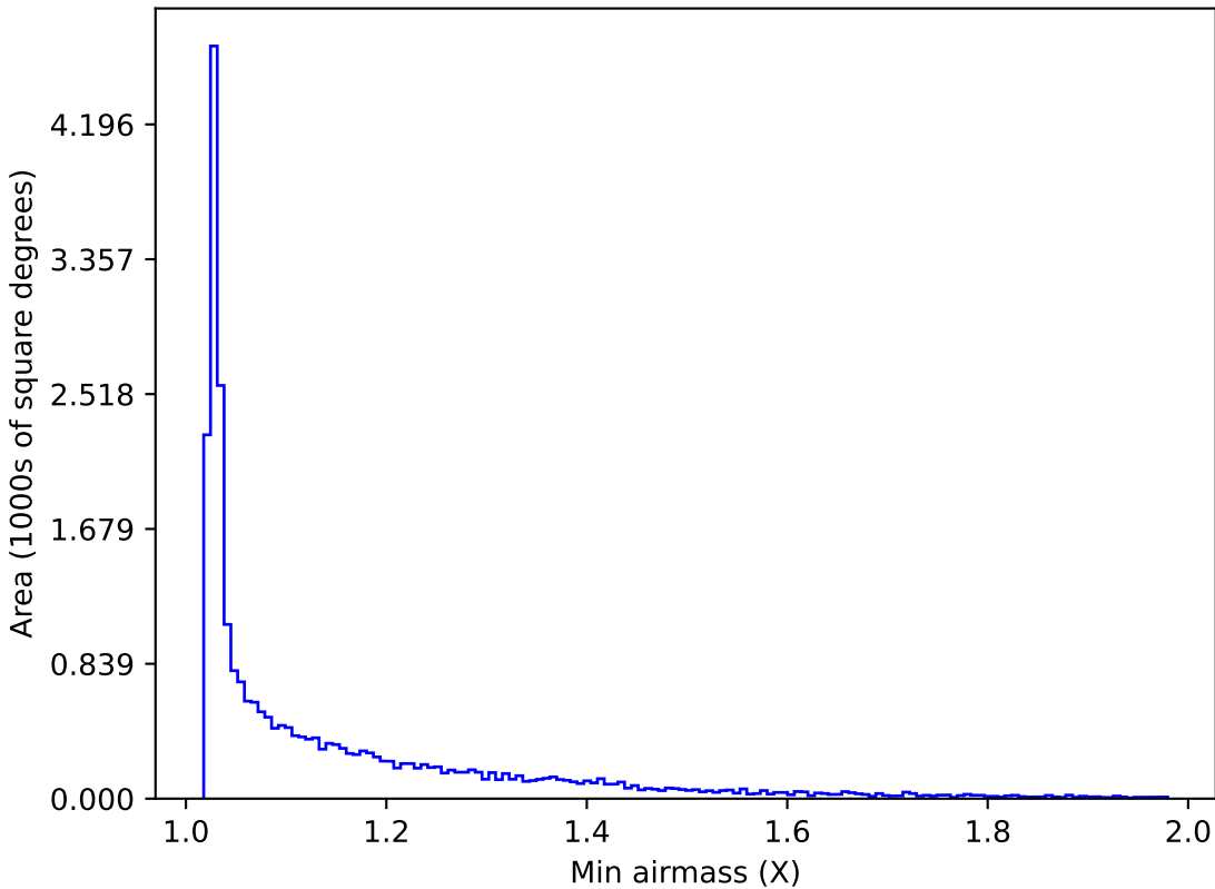
weather_cloudso35v3.4_10yrs All sky r band: Min airmass
