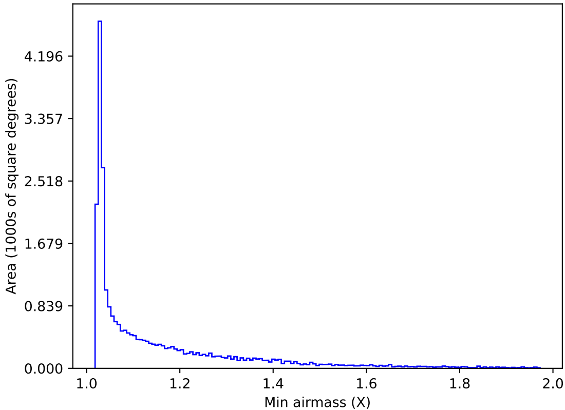
weather_cloudso35v3.4_10yrs All sky i band: Min airmass
