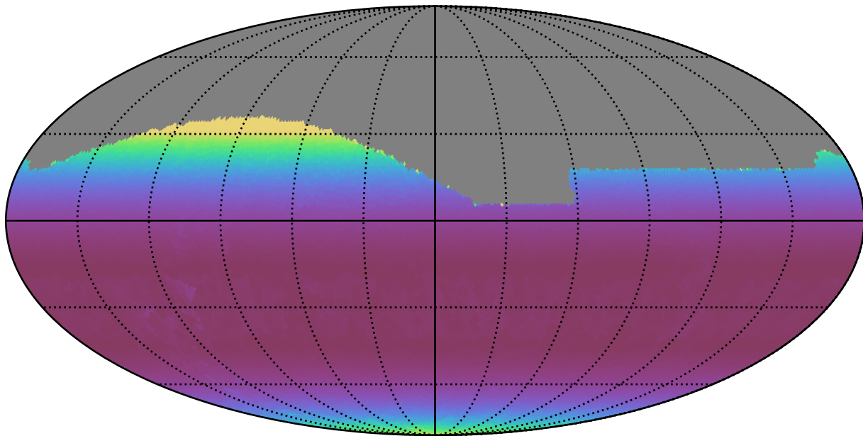
weather_cloudso35v3.4_10yrs All sky g band: Min airmass
