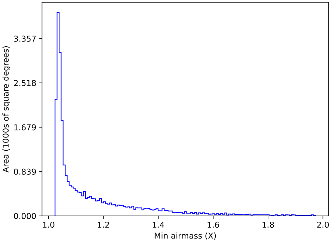
weather_cloudso35v3.4_10yrs All sky g band: Min airmass
