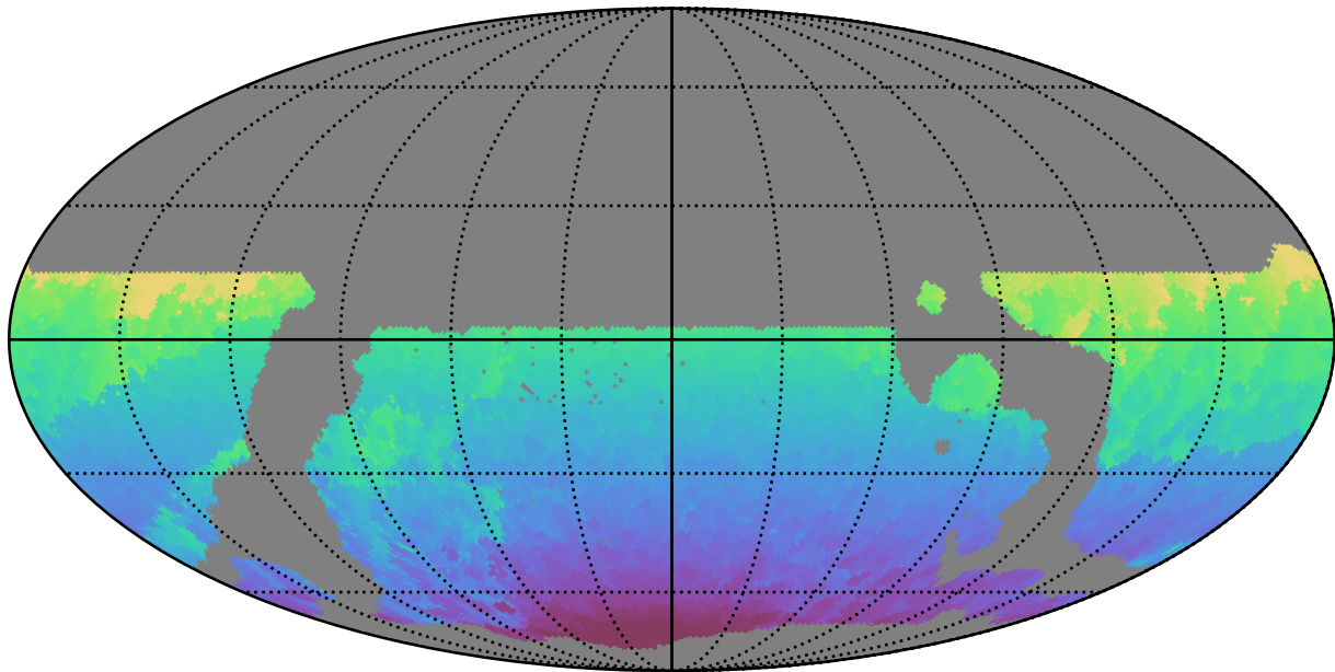
weather_cloudso35v3.4_10yrs WFD all bands: Min HA
