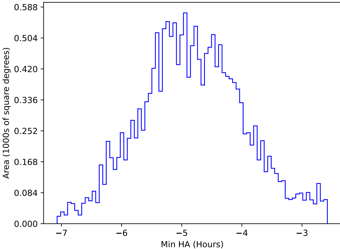
weather_cloudso35v3.4_10yrs WFD all bands: Min HA
