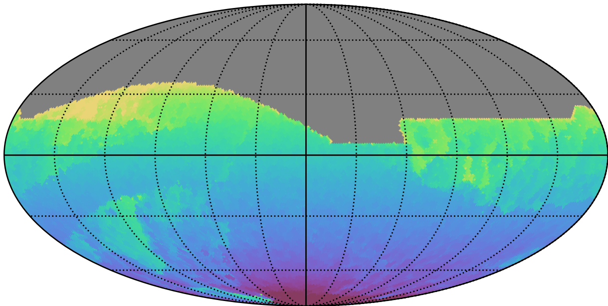
weather_cloudso35v3.4_10yrs All sky all bands: Min HA
