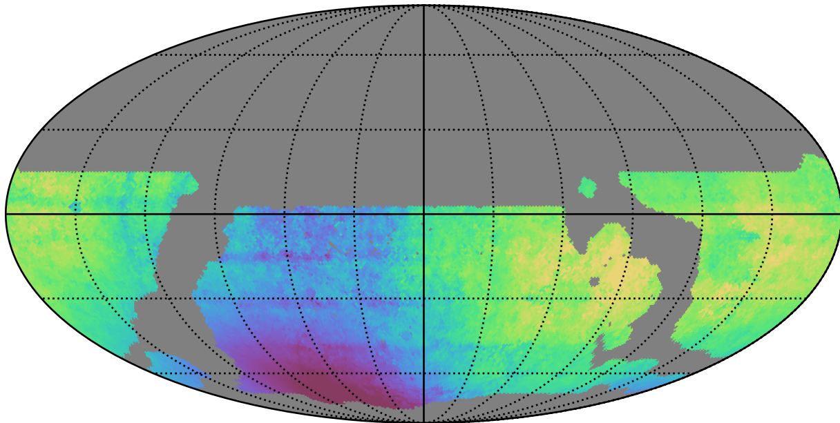
weather_cloudso35v3.4_10yrs WFD z band: Median solarElong
