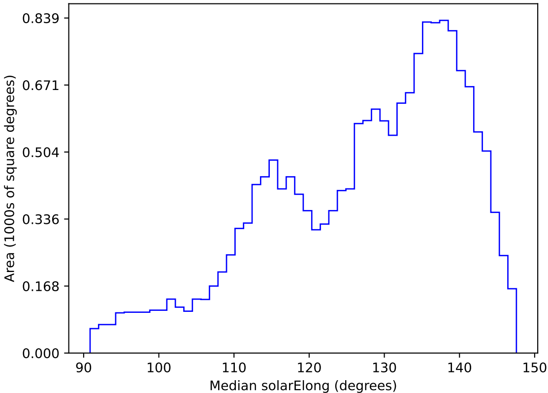
weather_cloudso35v3.4_10yrs WFD z band: Median solarElong
