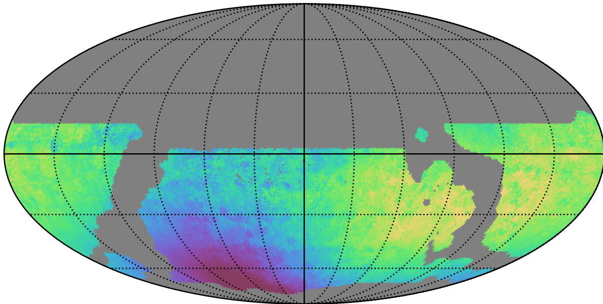
weather_cloudso35v3.4_10yrs WFD y band: Median solarElong
