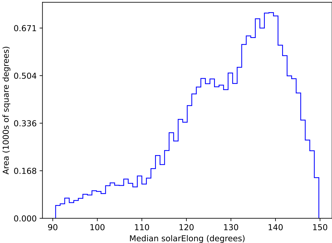
weather_cloudso35v3.4_10yrs WFD y band: Median solarElong
