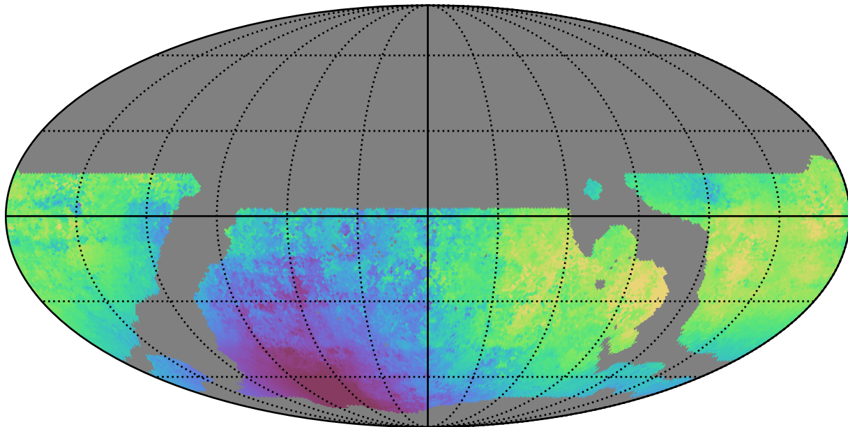
weather_cloudso35v3.4_10yrs WFD u band: Median solarElong
