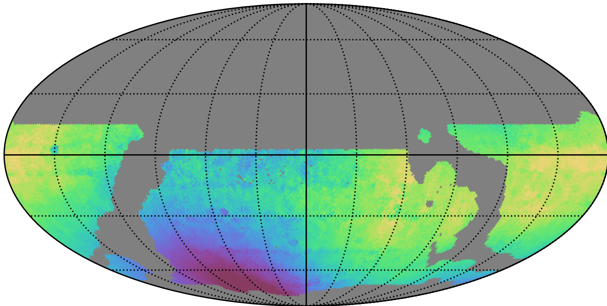
weather_cloudso35v3.4_10yrs WFD r band: Median solarElong
