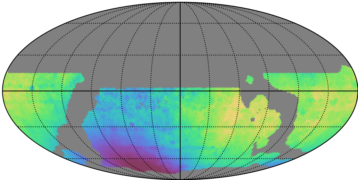
weather_cloudso35v3.4_10yrs WFD i band: Median solarElong
