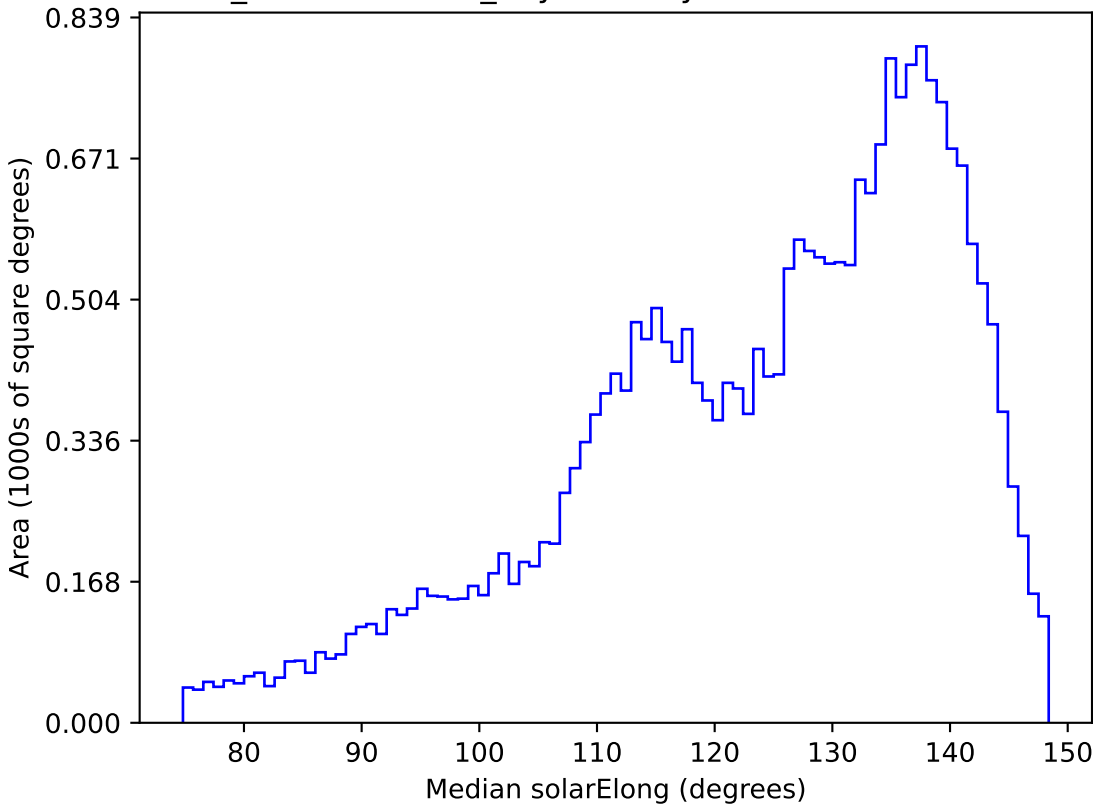
weather_cloudso35v3.4_10yrs All sky z band: Median solarElong
