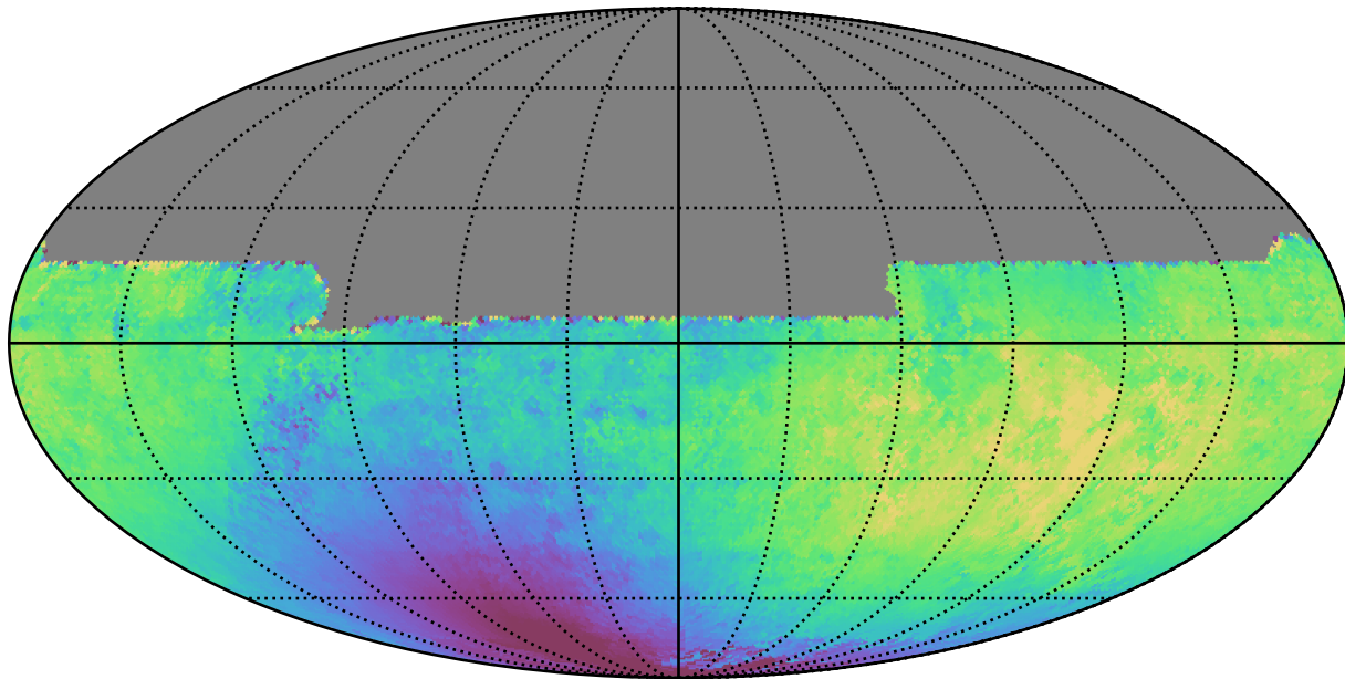
weather_cloudso35v3.4_10yrs All sky y band: Median solarElong
