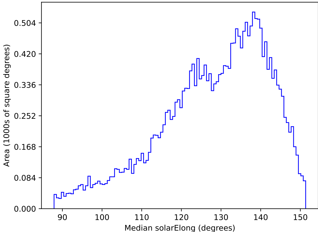
weather_cloudso35v3.4_10yrs All sky y band: Median solarElong
