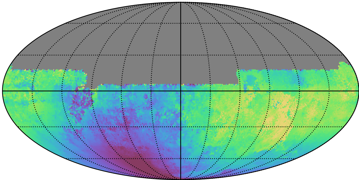
weather_cloudso35v3.4_10yrs All sky u band: Median solarElong
