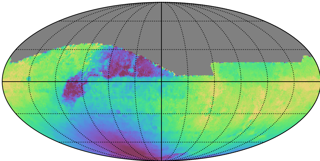
weather_cloudso35v3.4_10yrs All sky r band: Median solarElong
