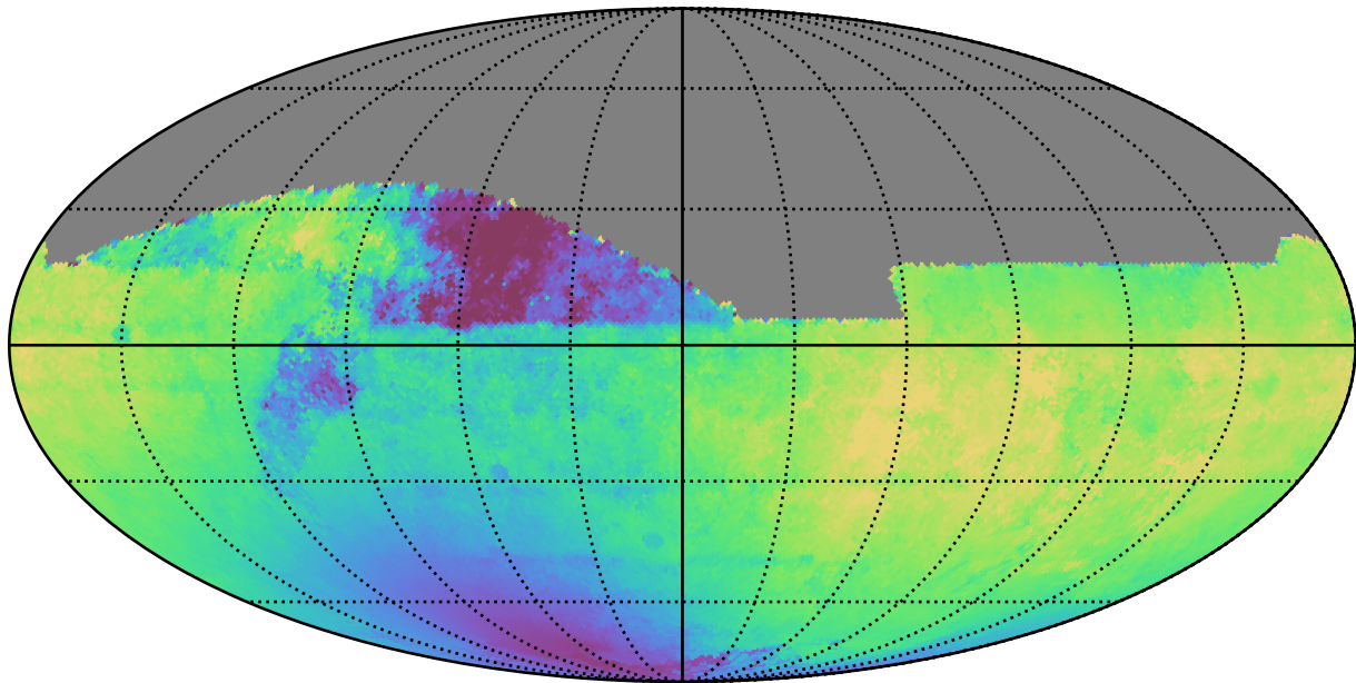
weather_cloudso35v3.4_10yrs All sky i band: Median solarElong
