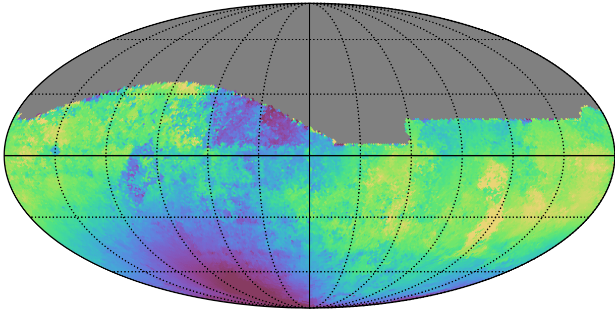
weather_cloudso35v3.4_10yrs All sky g band: Median solarElong
