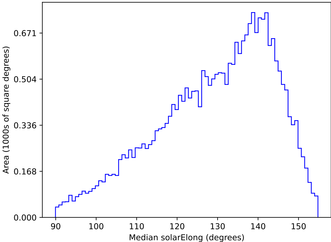
weather_cloudso35v3.4_10yrs All sky g band: Median solarElong
