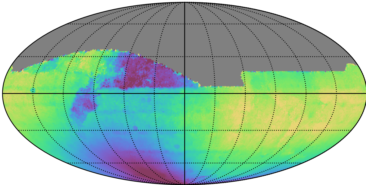
weather_cloudso35v3.4_10yrs All sky all bands: Median solarElong
