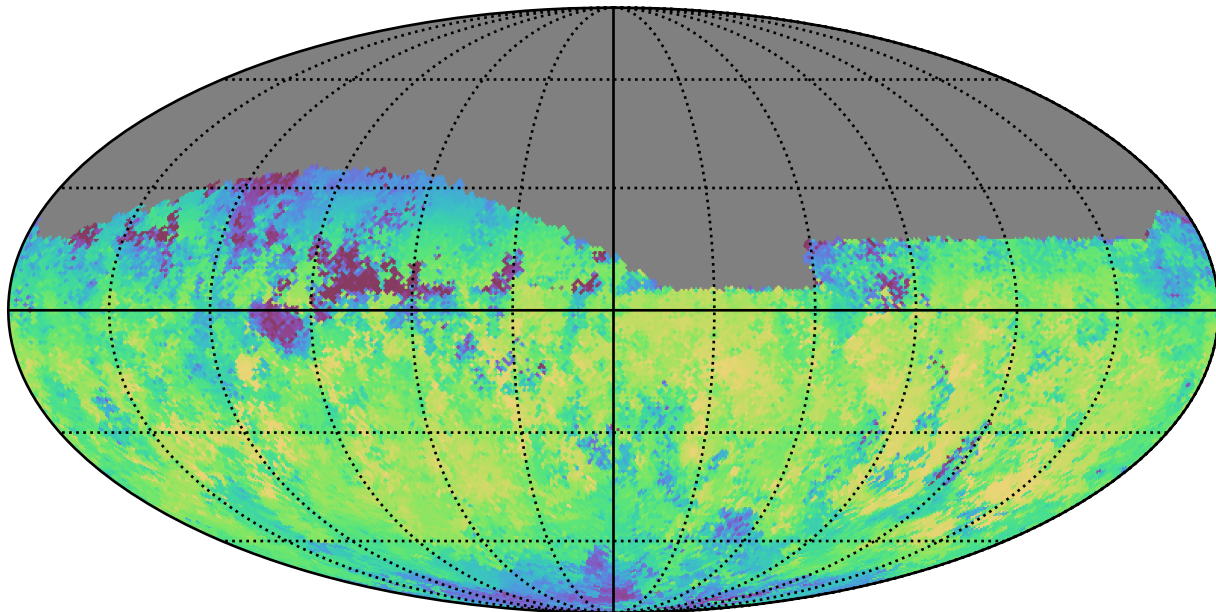
weather_cloudso35v3.4_10yrs Yr 1 z band: Median skyBrightness
