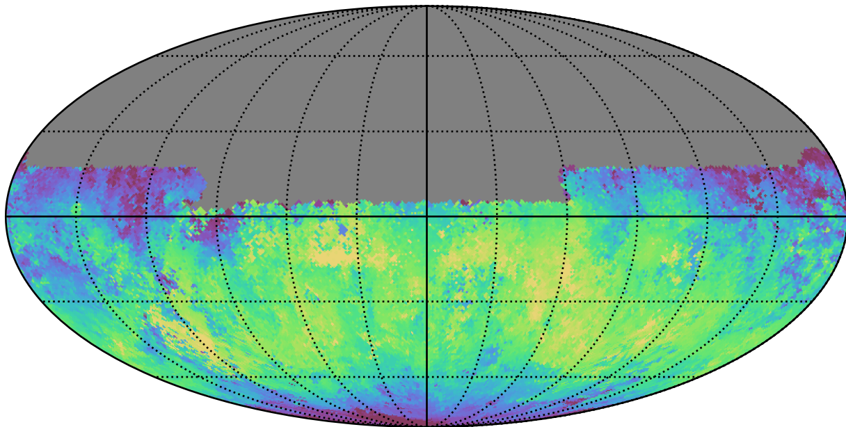
weather_cloudso35v3.4_10yrs Yr 1 y band: Median skyBrightness
