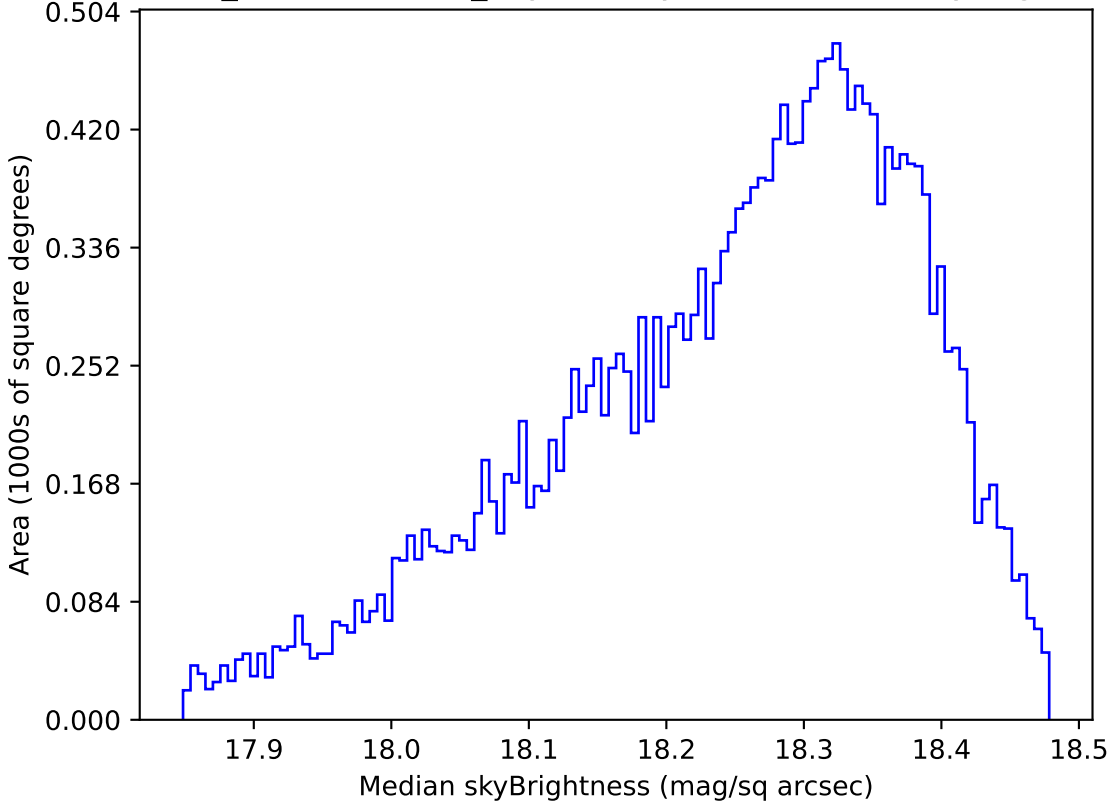
weather_cloudso35v3.4_10yrs Yr 1 y band: Median skyBrightness
