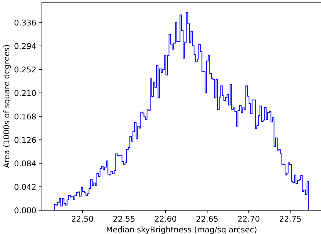
weather_cloudso35v3.4_10yrs Yr 1 u band: Median skyBrightness
