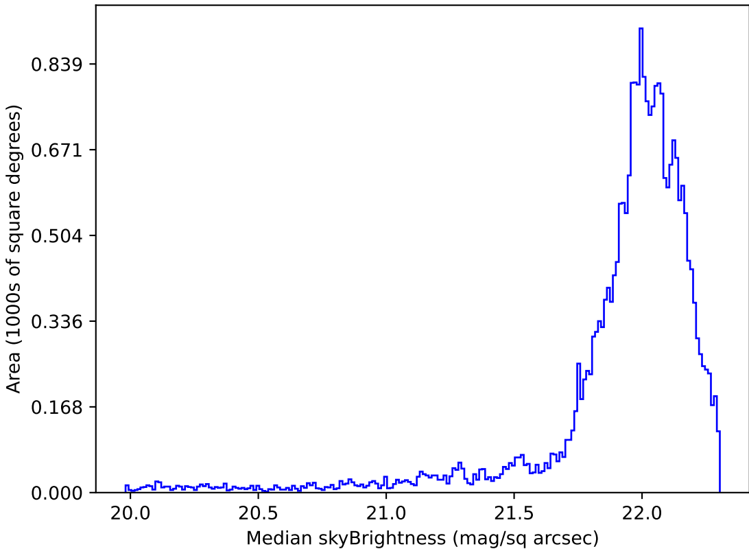
weather_cloudso35v3.4_10yrs Yr 1 g band: Median skyBrightness
