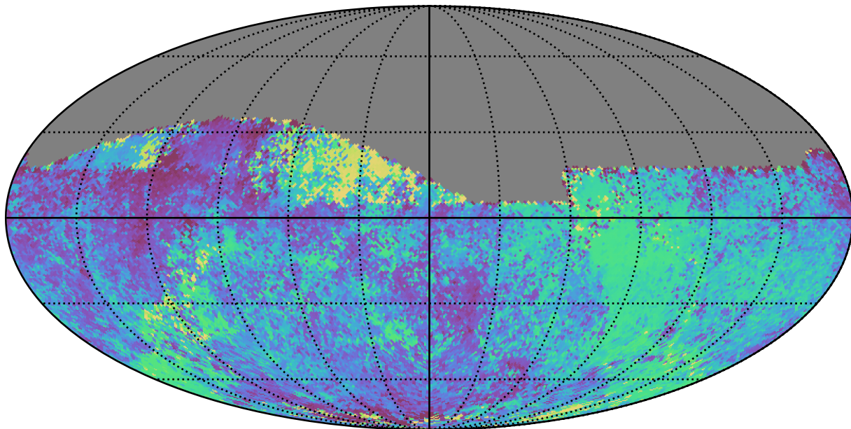
weather_cloudso35v3.4_10yrs Yr 1 all bands: Median skyBrightness
