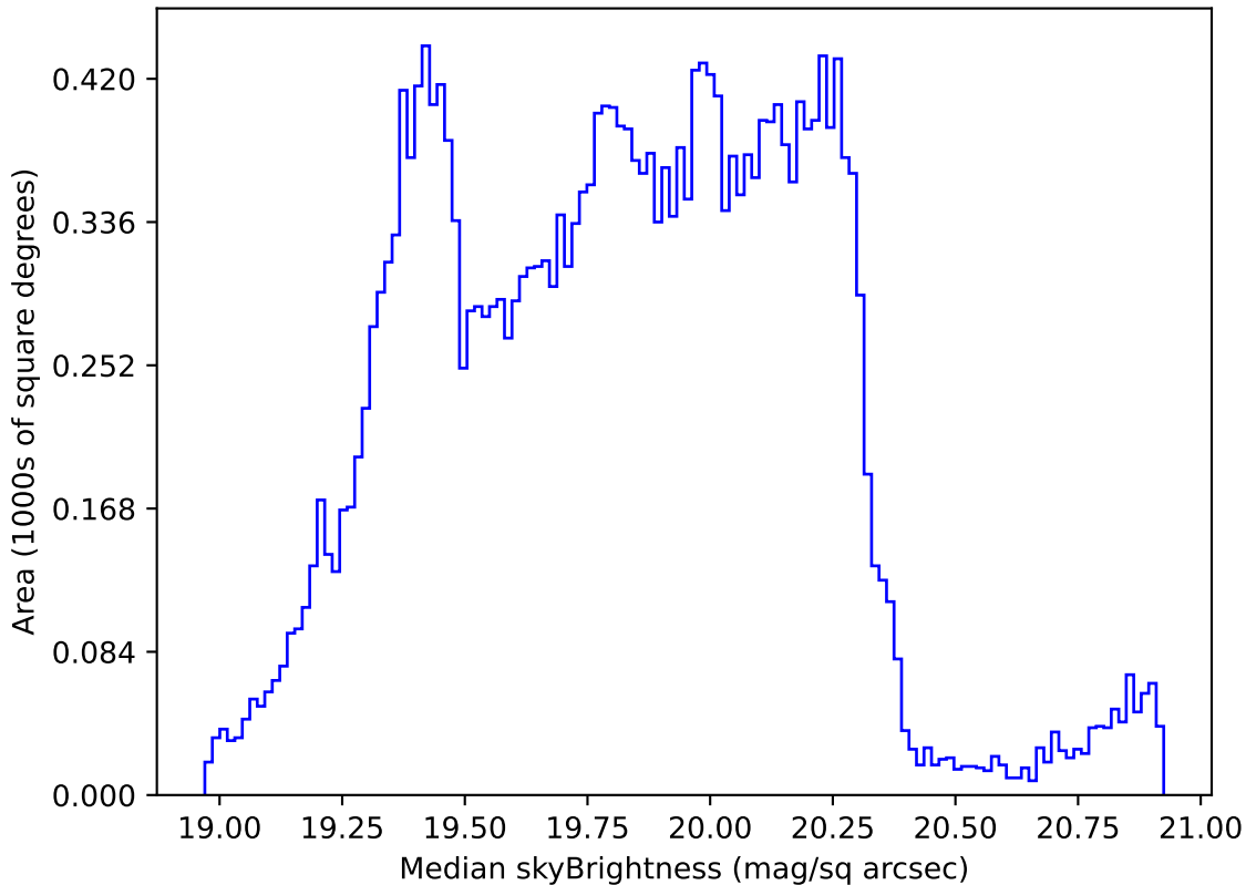
weather_cloudso35v3.4_10yrs Yr 1 all bands: Median skyBrightness
