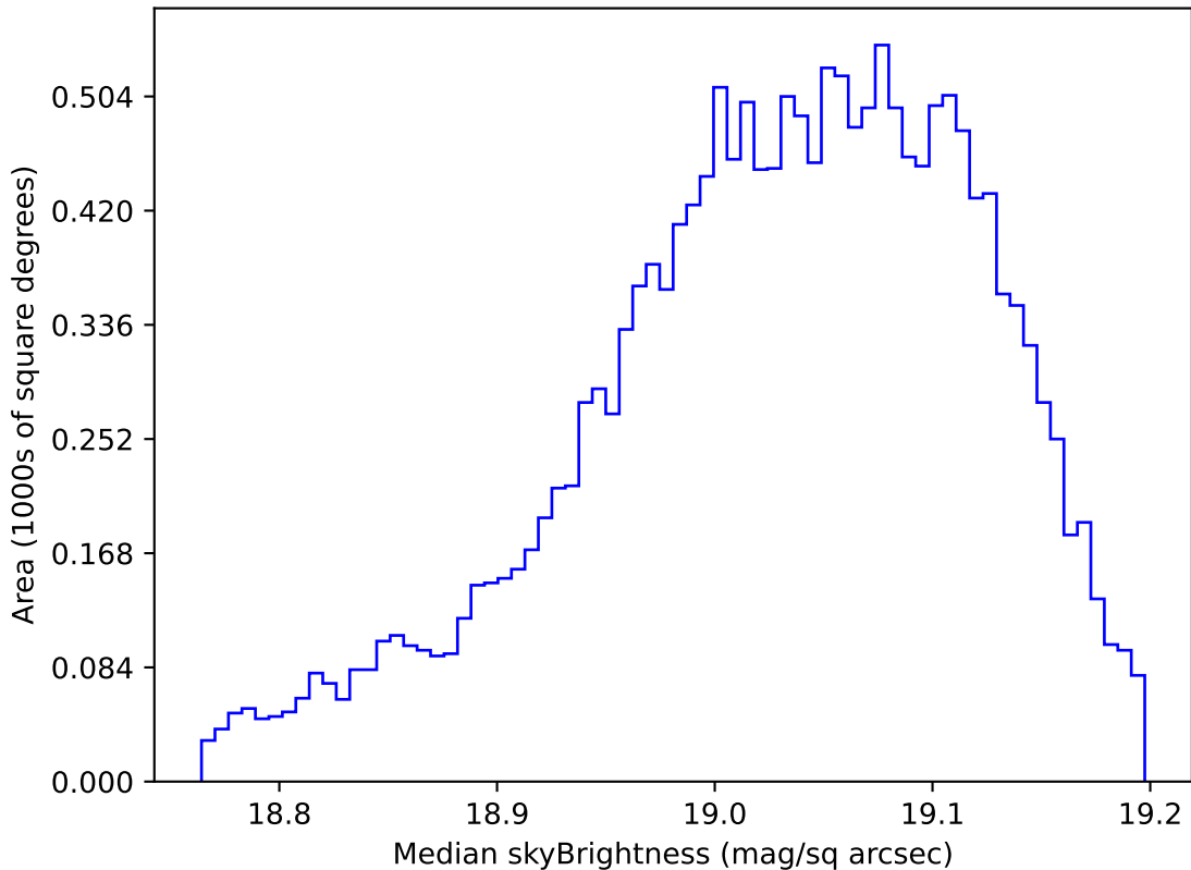
weather_cloudso35v3.4_10yrs WFD z band: Median skyBrightness
