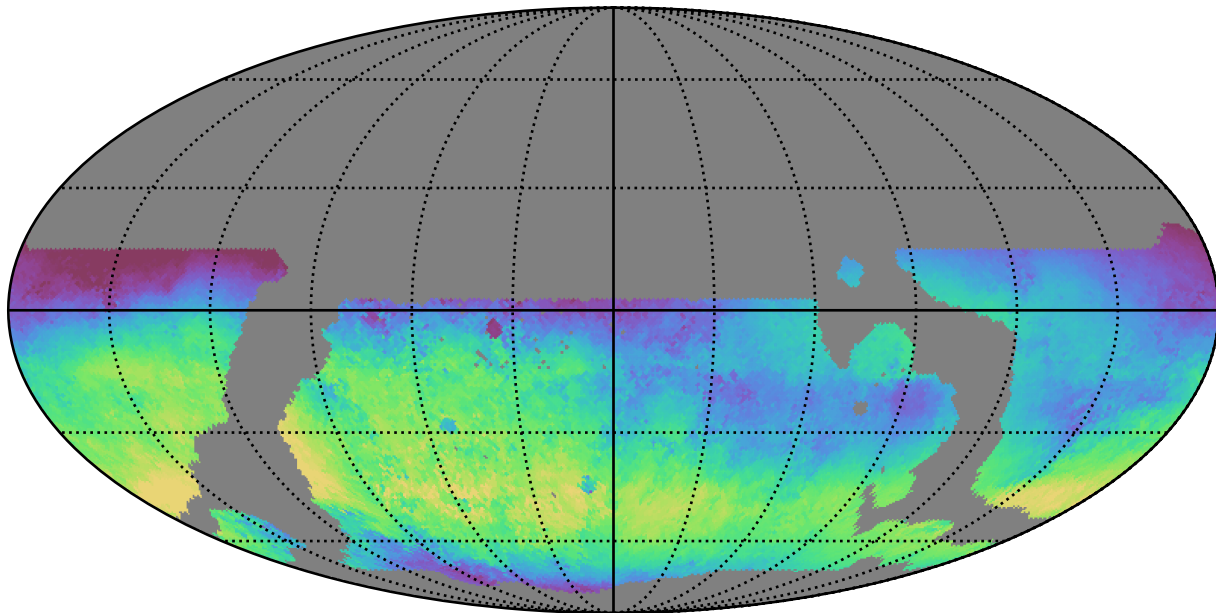
weather_cloudso35v3.4_10yrs WFD u band: Median skyBrightness
