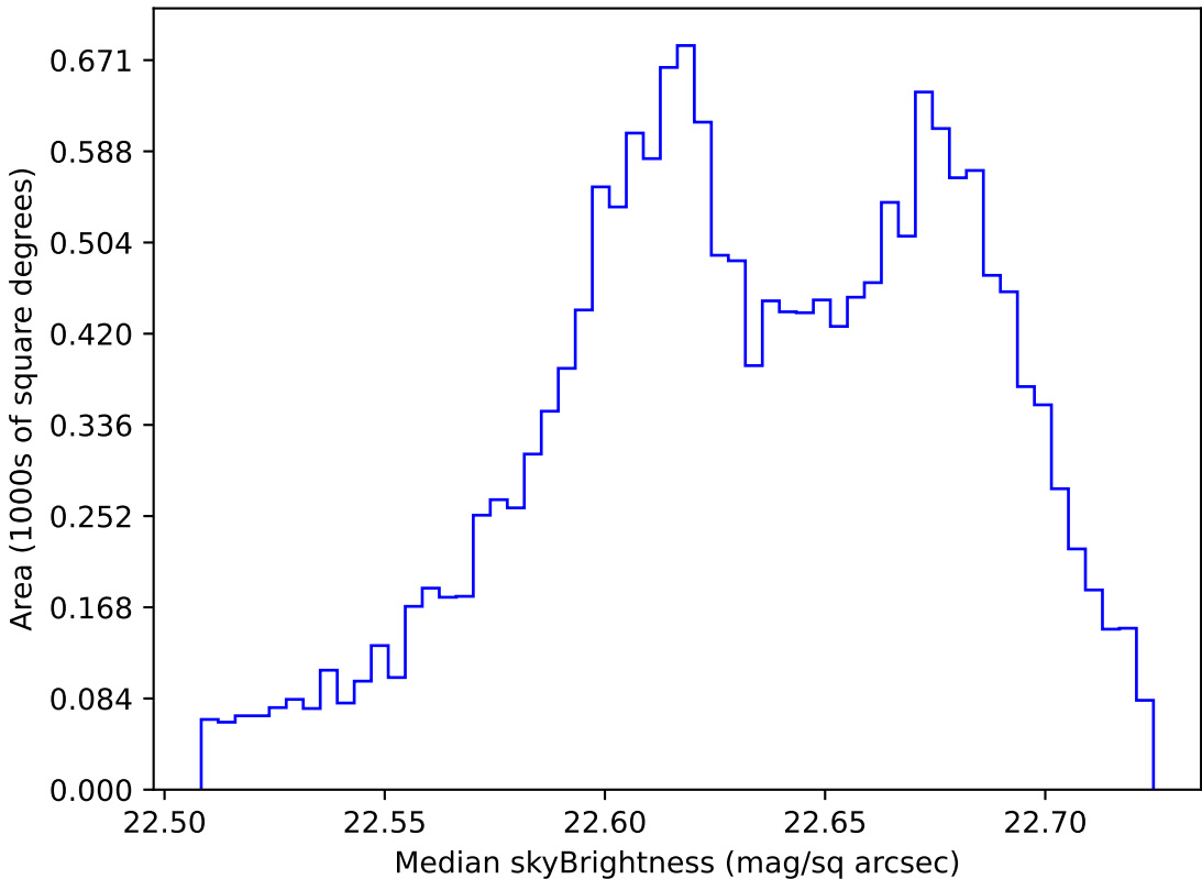
weather_cloudso35v3.4_10yrs WFD u band: Median skyBrightness
