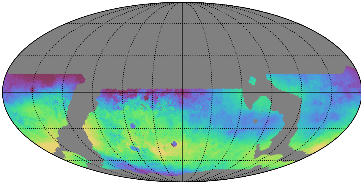
weather_cloudso35v3.4_10yrs WFD r band: Median skyBrightness
