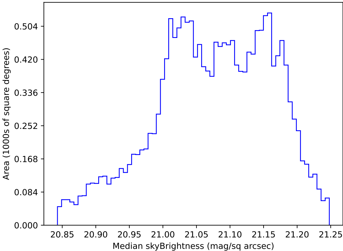
weather_cloudso35v3.4_10yrs WFD r band: Median skyBrightness
