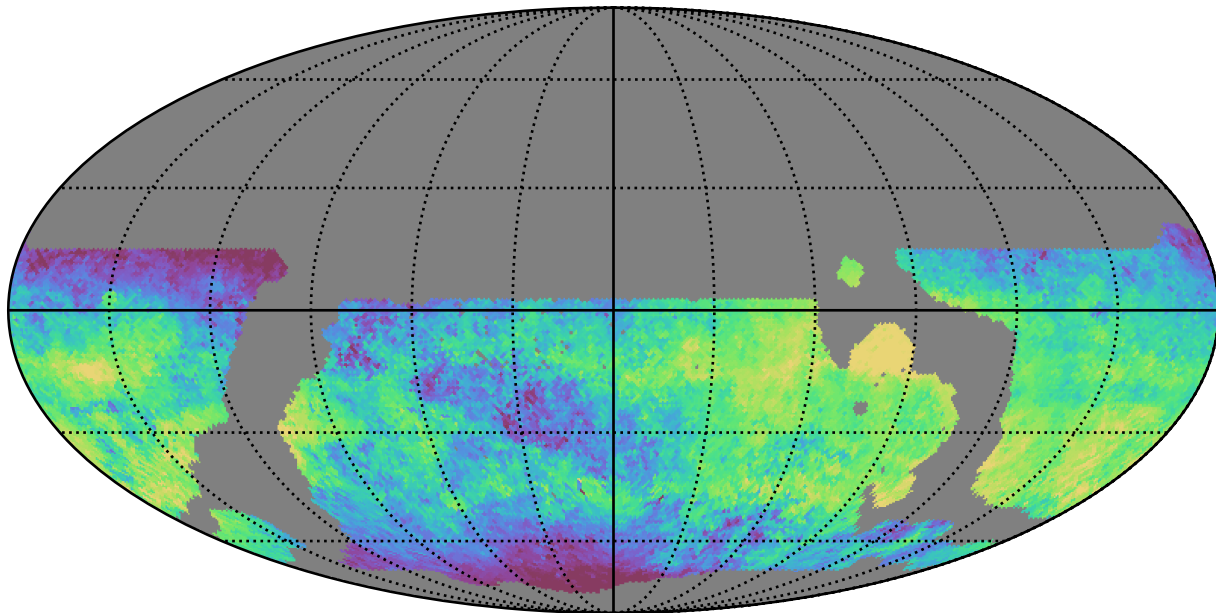
weather_cloudso35v3.4_10yrs WFD i band: Median skyBrightness
