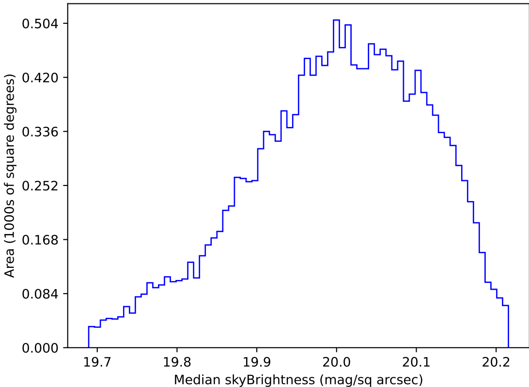
weather_cloudso35v3.4_10yrs WFD i band: Median skyBrightness
