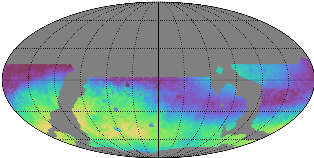
weather_cloudso35v3.4_10yrs WFD g band: Median skyBrightness
