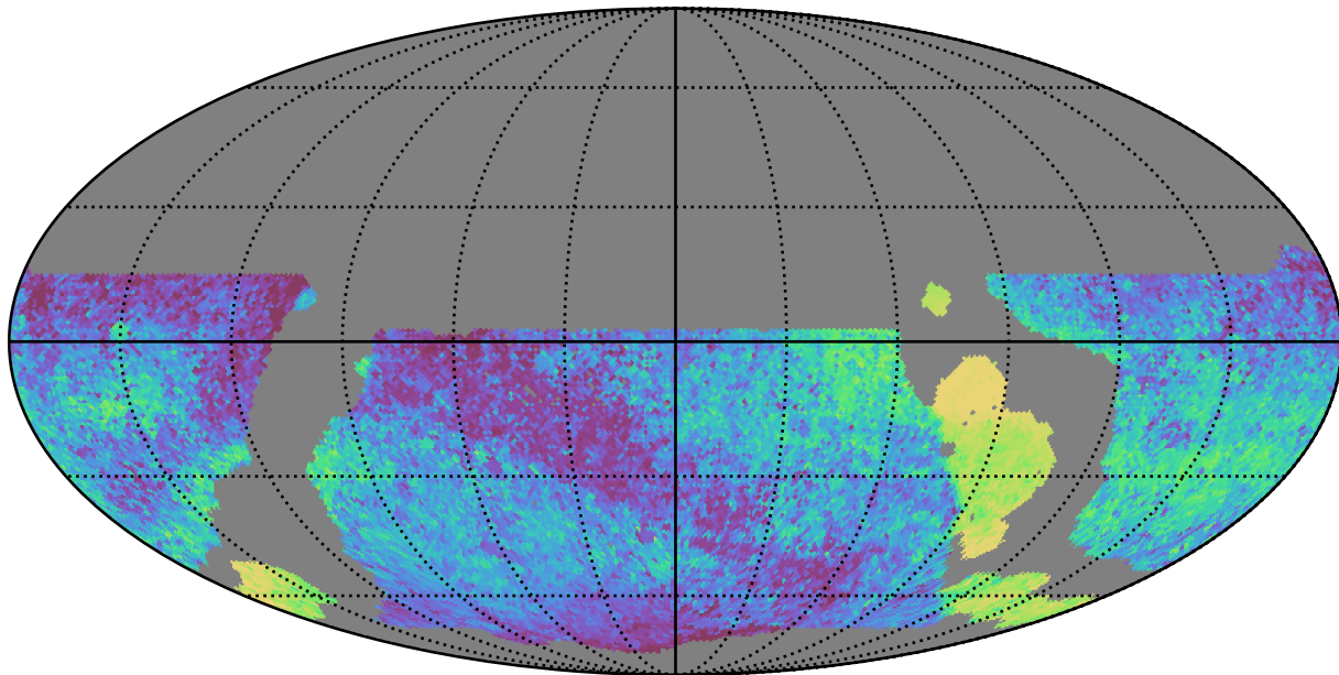
weather_cloudso35v3.4_10yrs WFD all bands: Median skyBrightness
