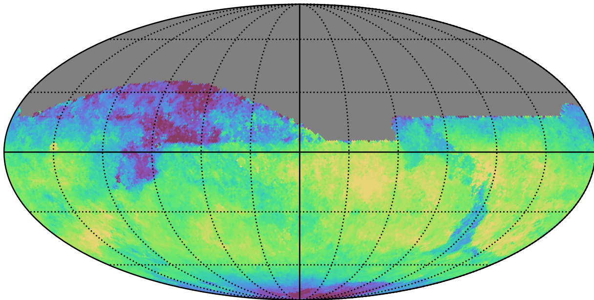
weather_cloudso35v3.4_10yrs All sky z band: Median skyBrightness
