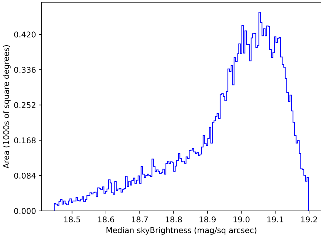
weather_cloudso35v3.4_10yrs All sky z band: Median skyBrightness
