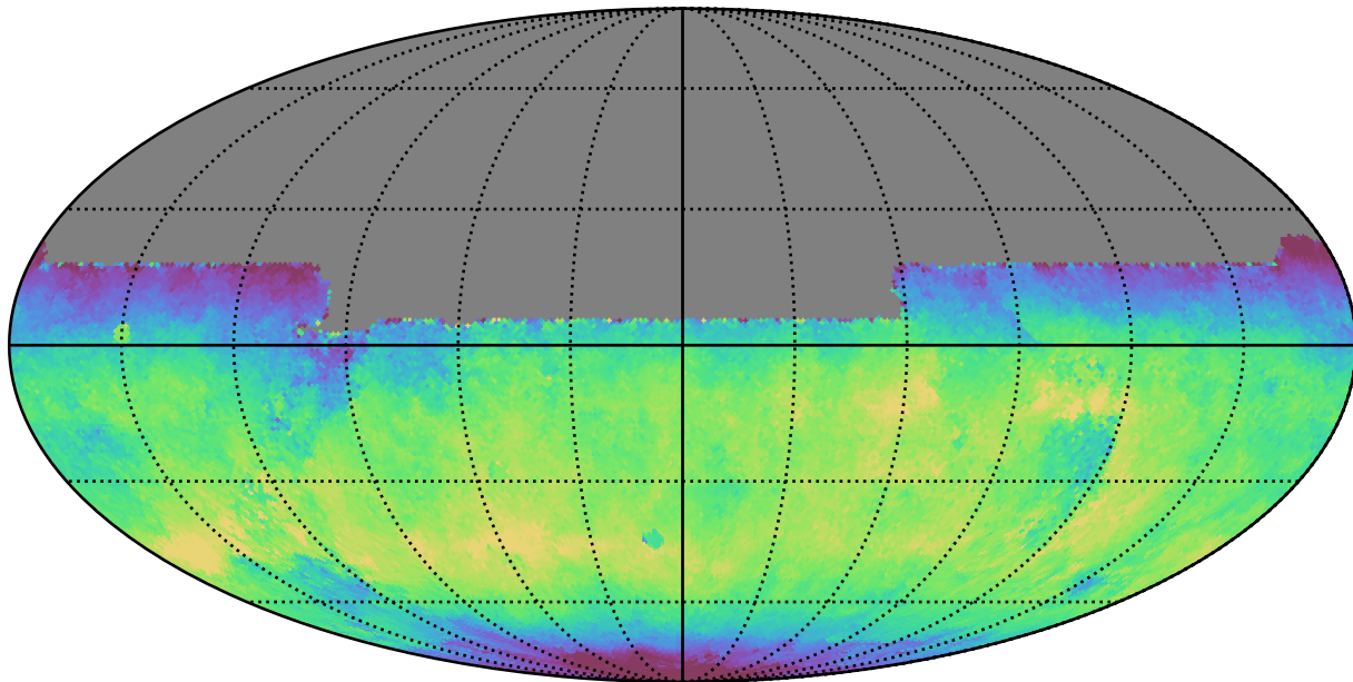
weather_cloudso35v3.4_10yrs All sky y band: Median skyBrightness
