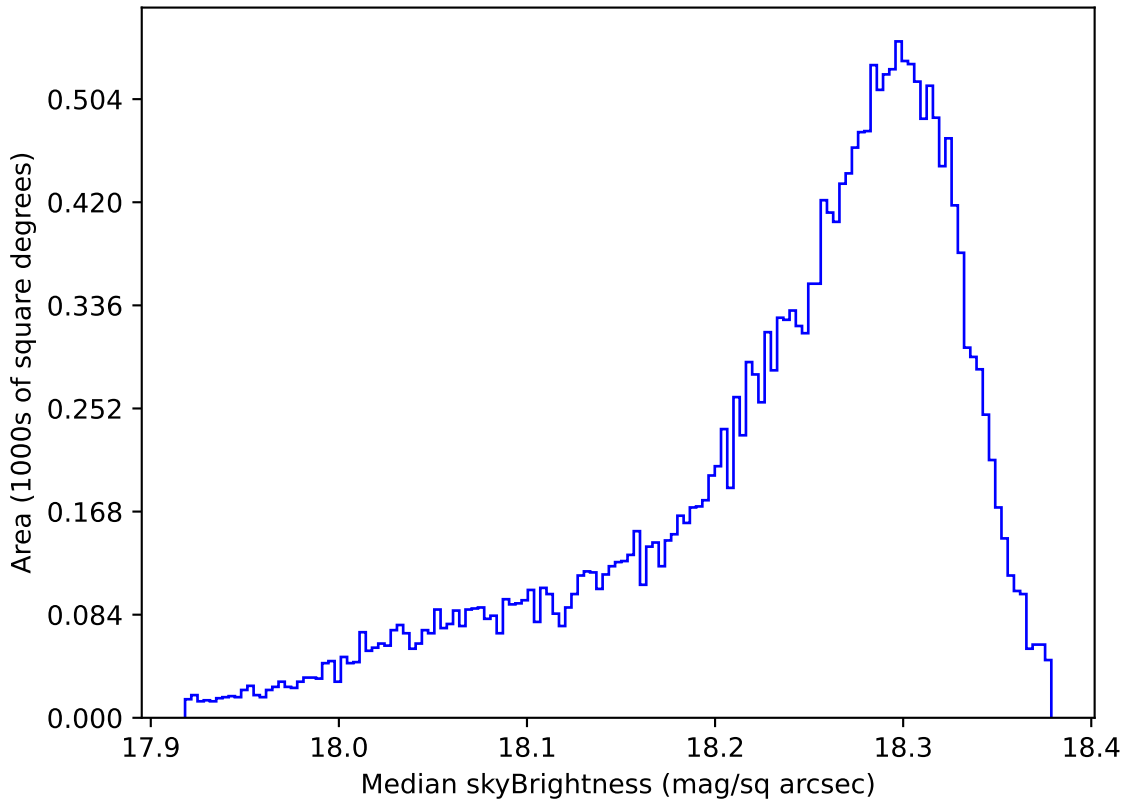
weather_cloudso35v3.4_10yrs All sky y band: Median skyBrightness
