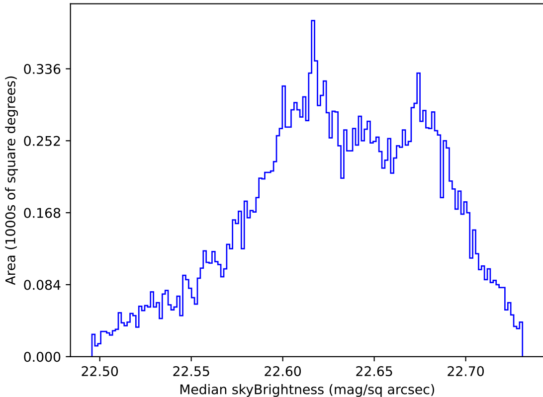
weather_cloudso35v3.4_10yrs All sky u band: Median skyBrightness
